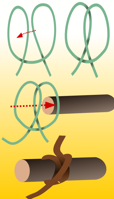
CLOVE HITCH
