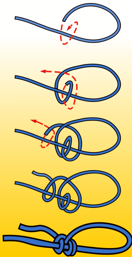
TAUGHT-LINE HITCH
